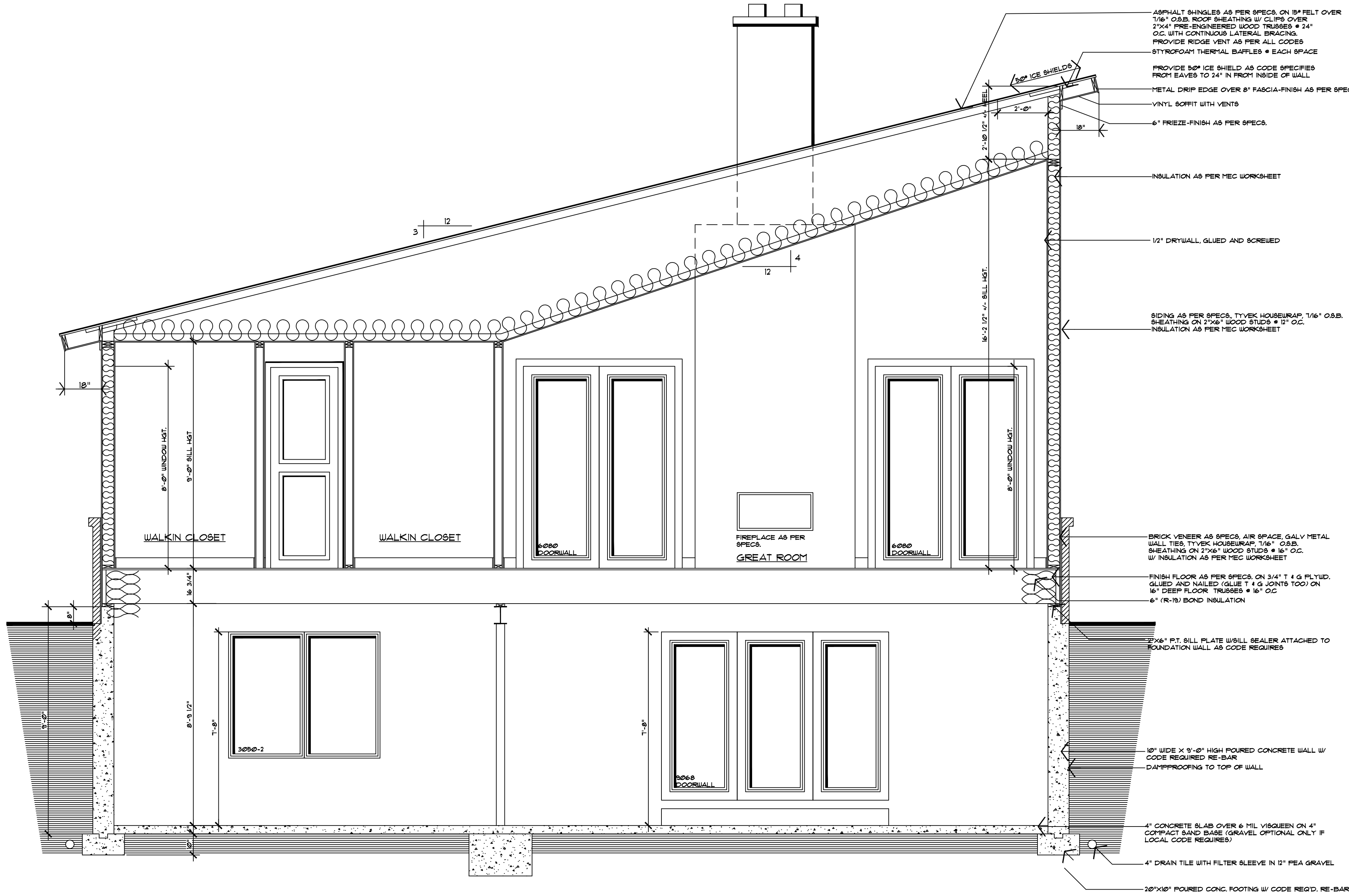
TRANSVERSE SECTION "4-A"
